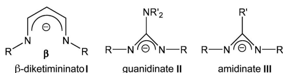
Scheme 1. Typical N,N' -chelating ligands.
